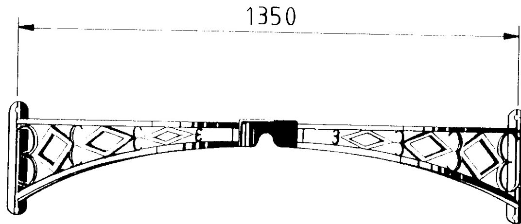
BOW BRACKET SMALL
