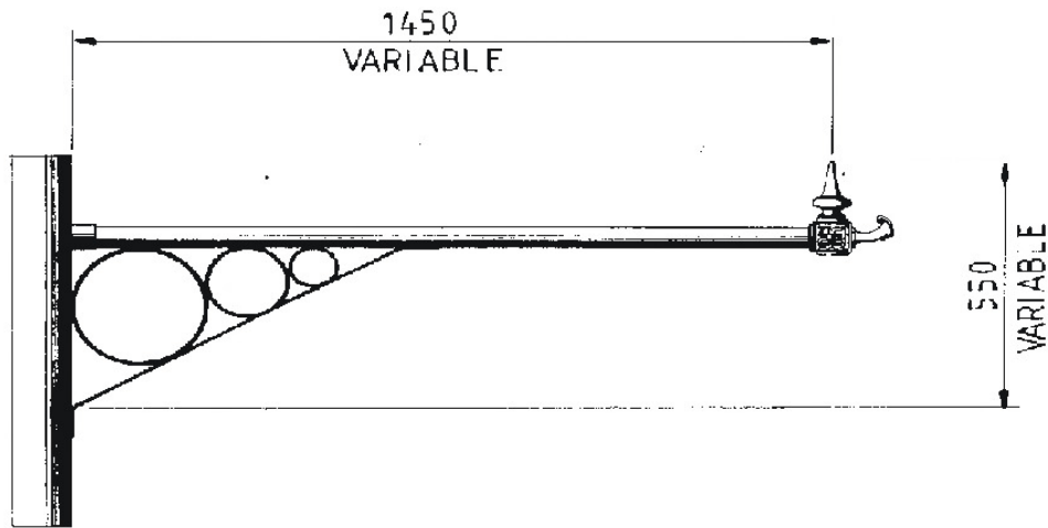
EDINBURGH COLUMN MOUNTING
