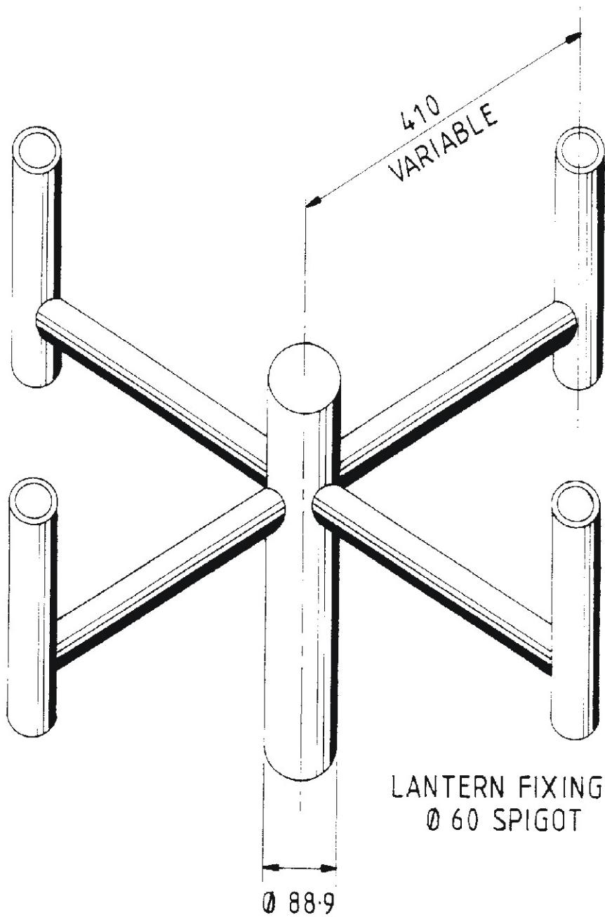
PLAIN ARM BRACKET X 4
