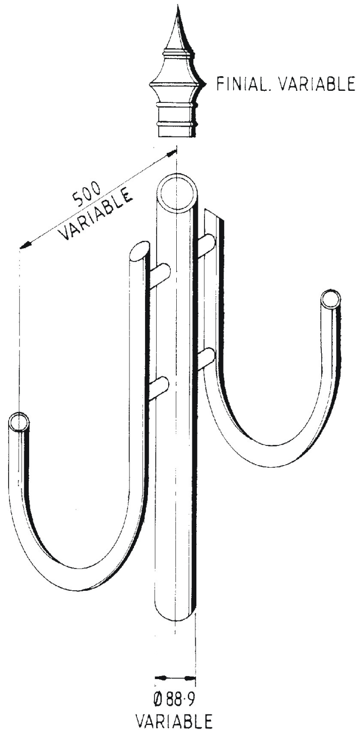
PLAIN 'U' ARM BRACKET X 2 CAN BE INVERTED
