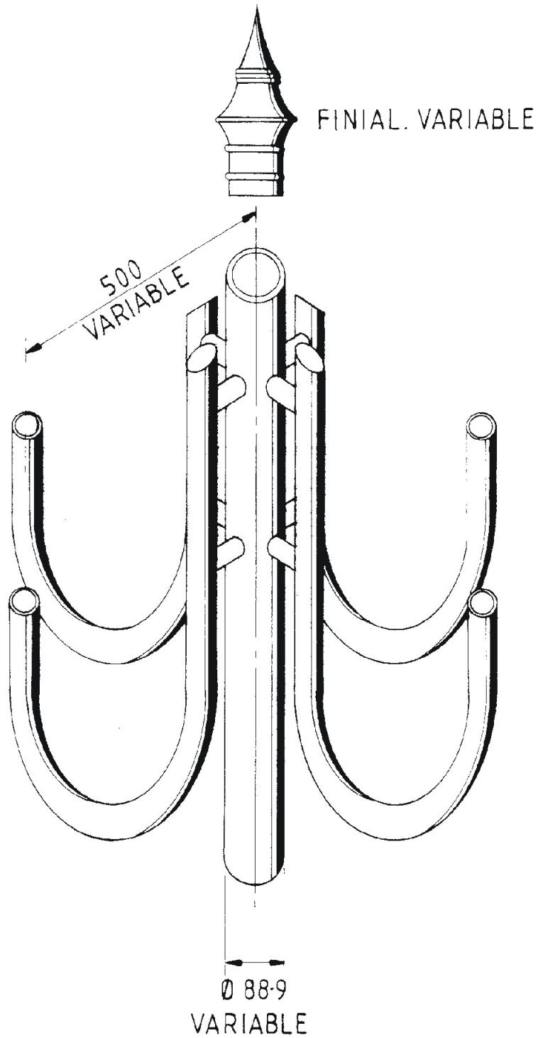
PLAIN 'U' ARM BRACKET X 4 CAN BE INVERTED
